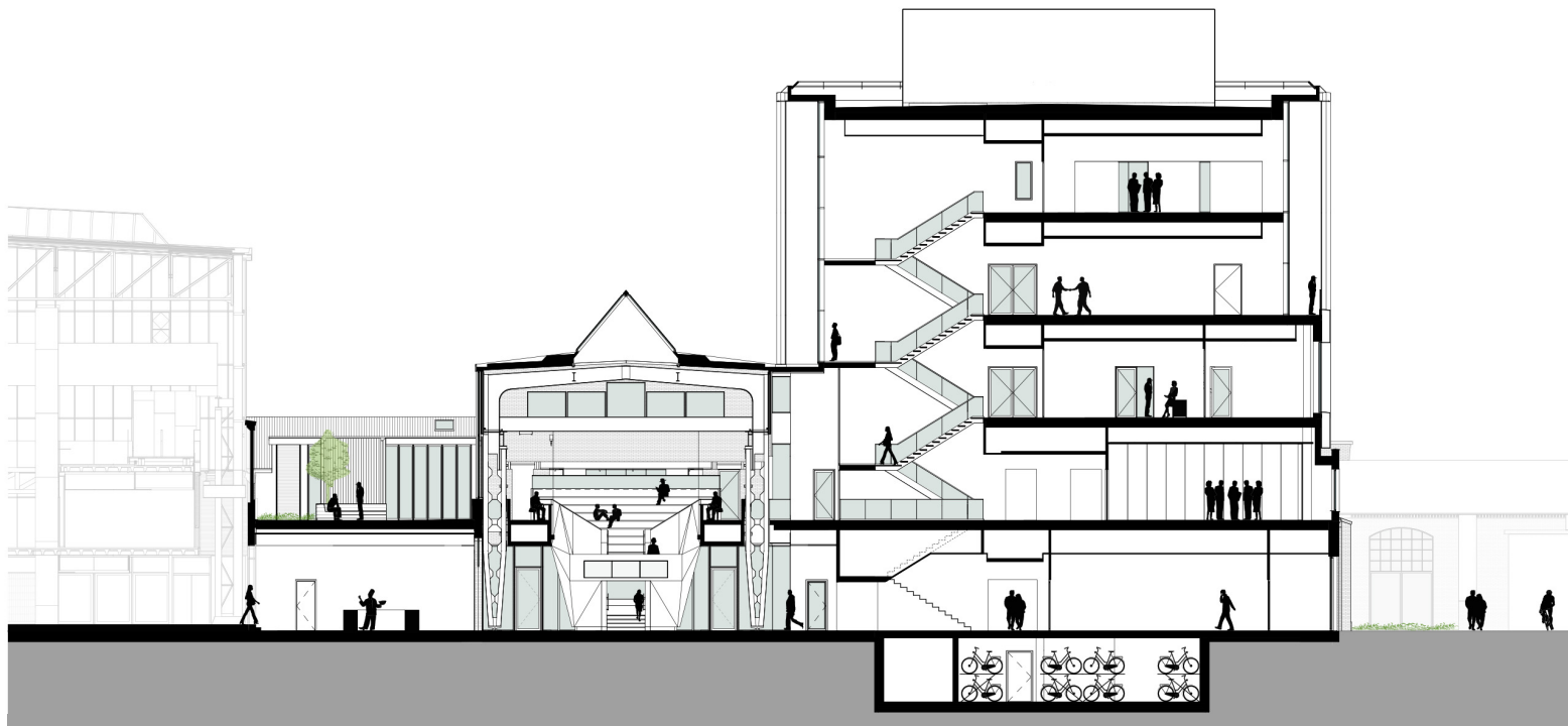
MindLabs dwarsdoorsnede
