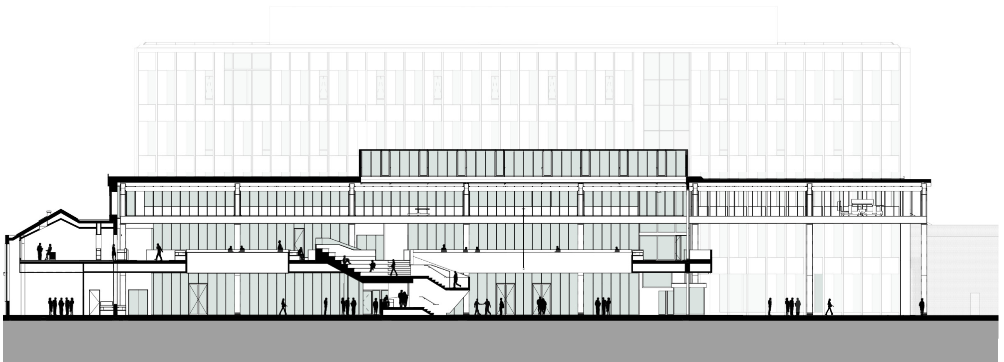
MindLabs langsdoorsnede
