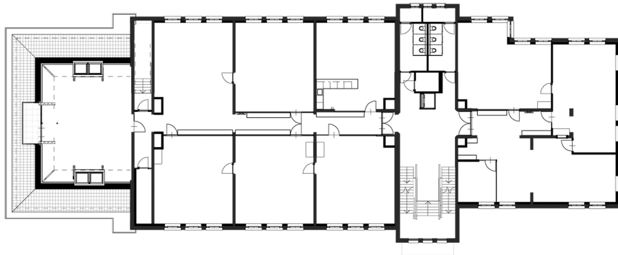
plattegrond +1
